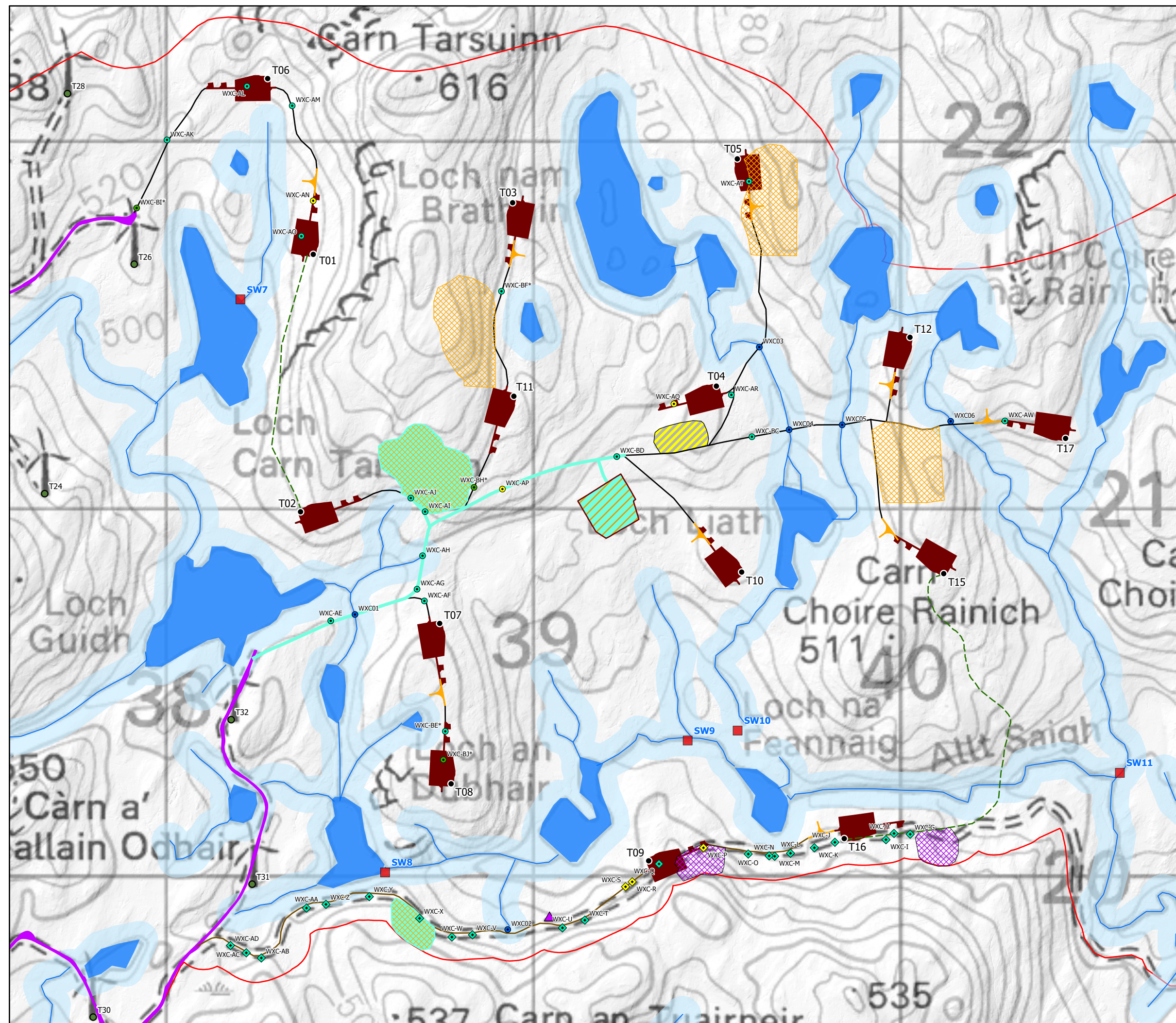
Figure 9.3 Hydrological Constraints & Watercourse Crossings - Proposed Varied Development Bhlaraidh Wind Farm Extension S36C EIA Report 2025 Proposed Varied Development
