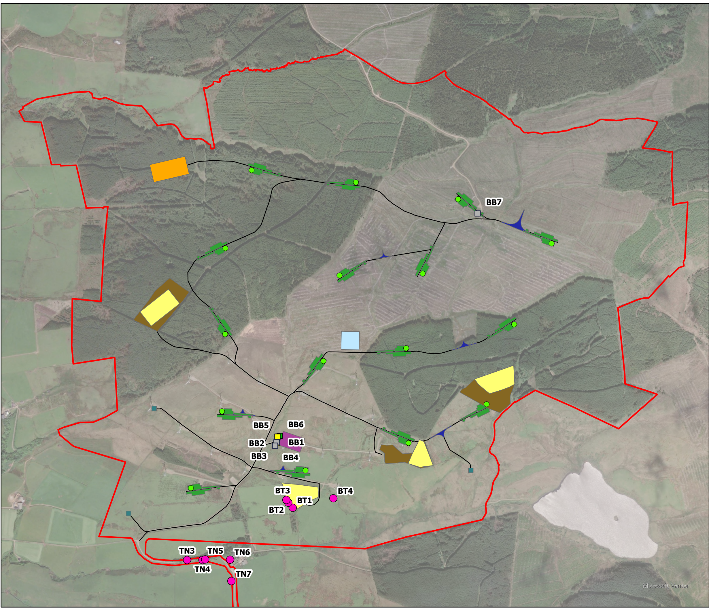
Figure 7.4 Bat Roost Assessment Tangy IV Wind Farm S36C EIA Report 2026 Proposed Varied Development
