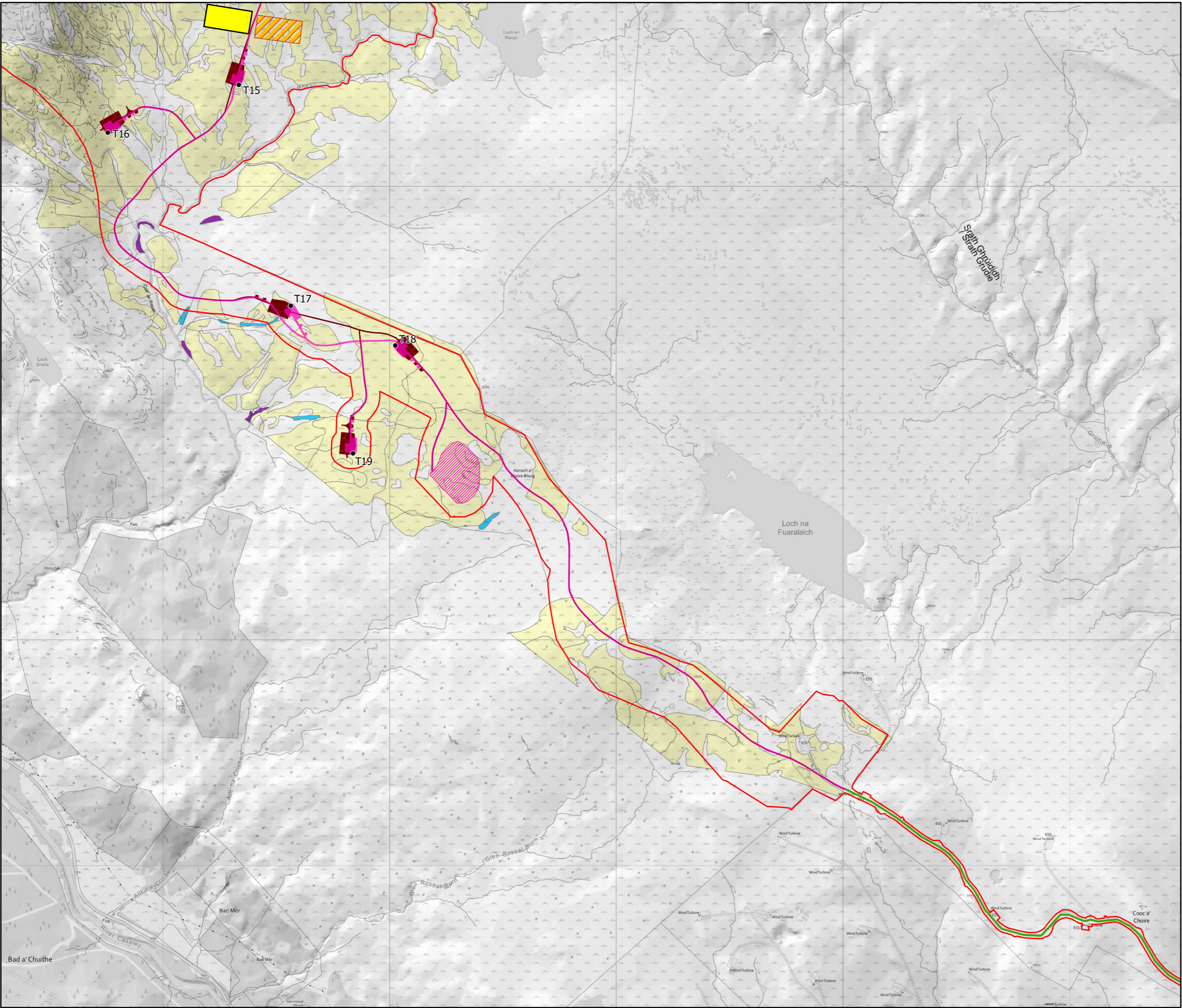
Figure 8.5b High GWDTE Potential (Based on NVC)
