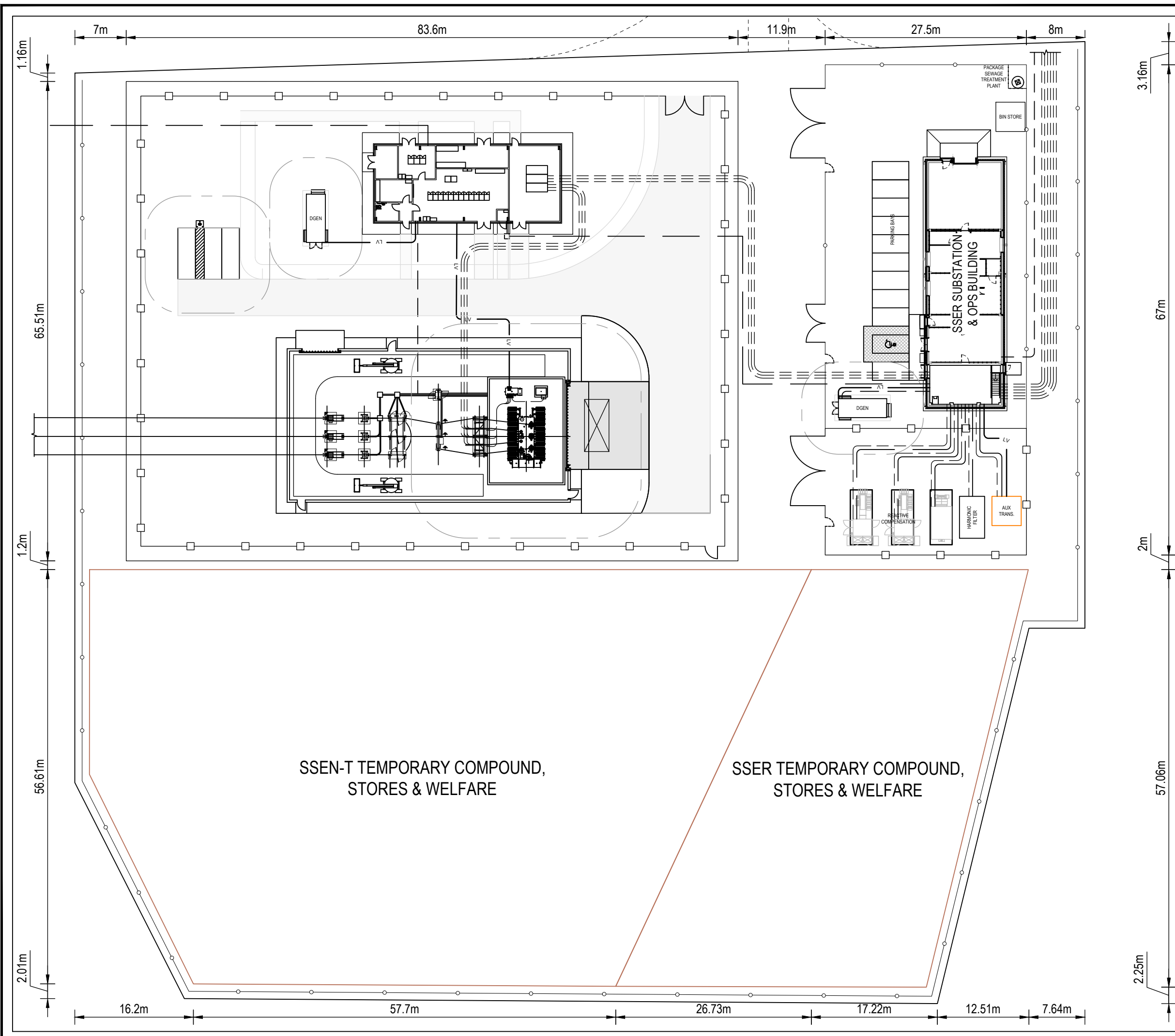
Figure 2.6 Indicative Substation Plan Layout
