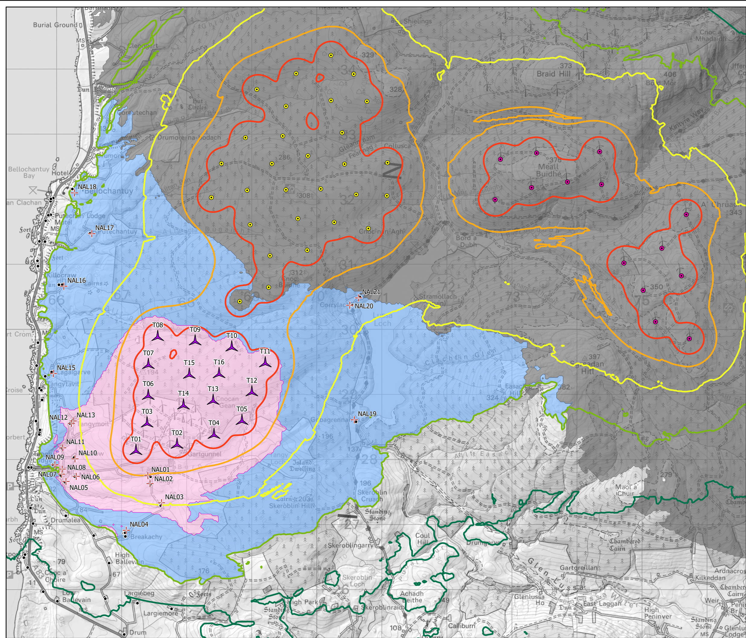
Figure 11.1a Cumulative Noise Contours and Receptors
