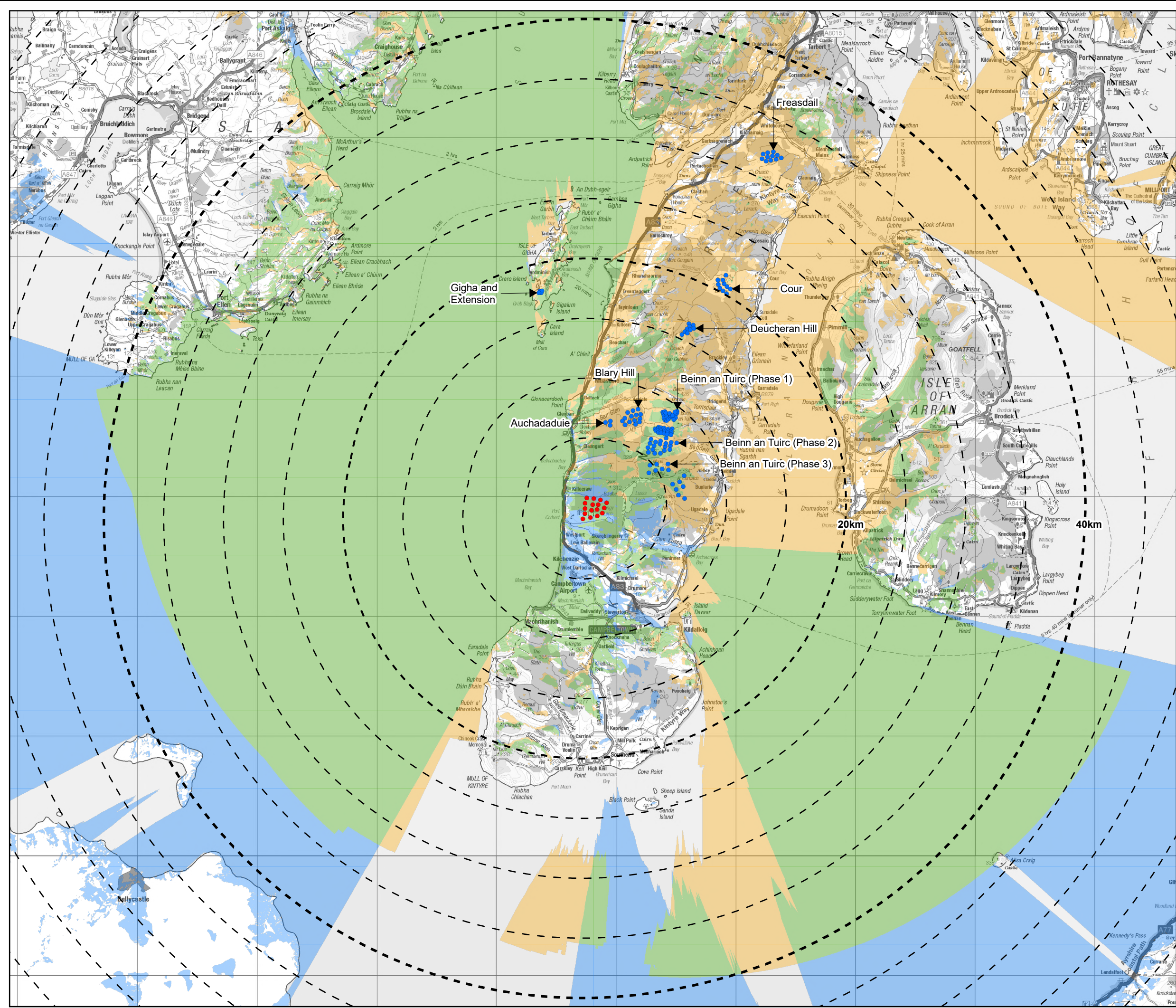
Figure V3a-5.12 Cumulative ZTV - Proposed Varied Development with All Operational Sites Tangy IV Wind Farm S36C EIA Report 2026 Proposed Varied Development
