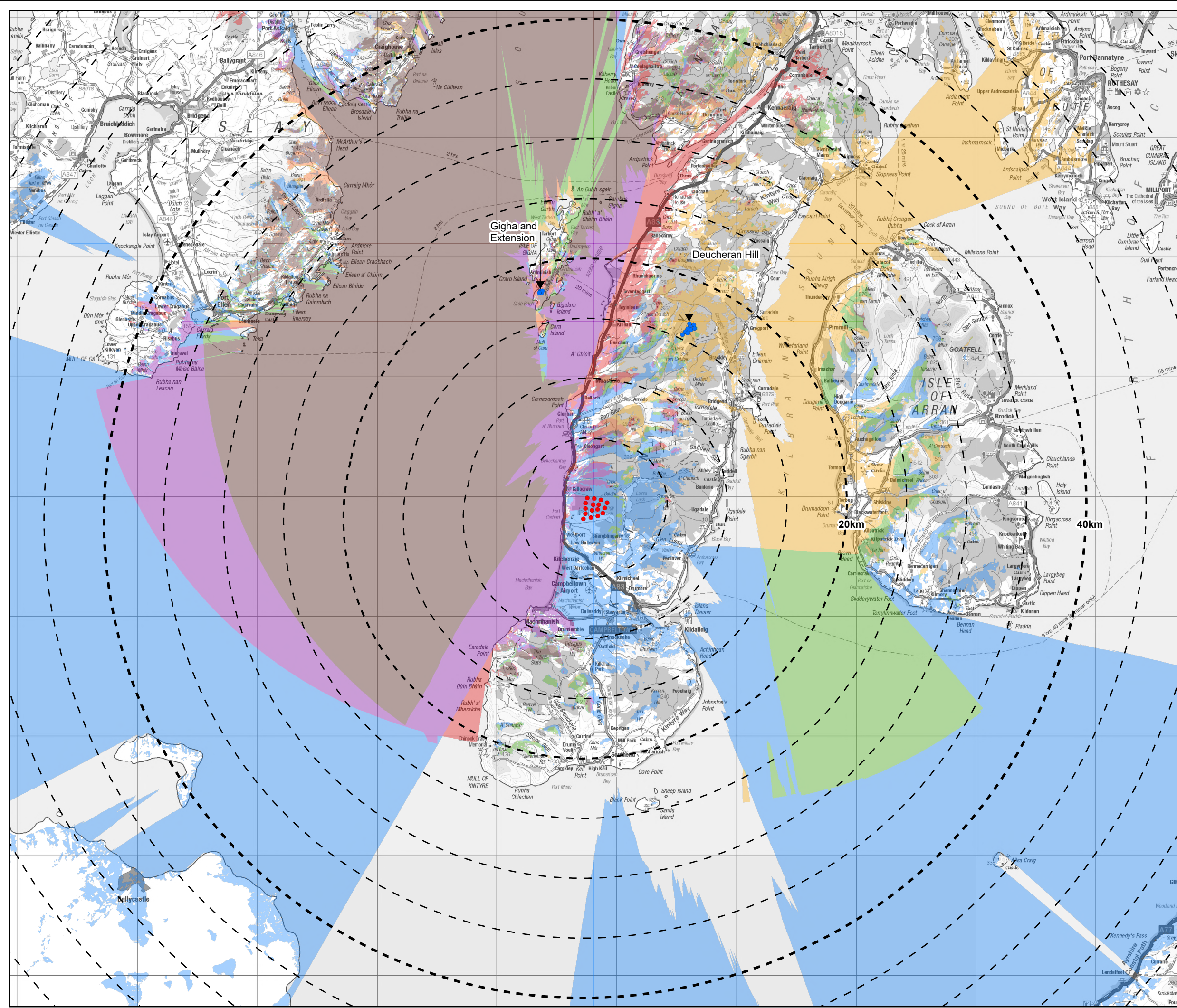
Figure V3a-5.19 Cumulative ZTV - Proposed Varied Development with Deucheran Hill and Gigha and Extension Tangy IV Wind Farm S36C EIA Report 2026 Proposed Varied Development
