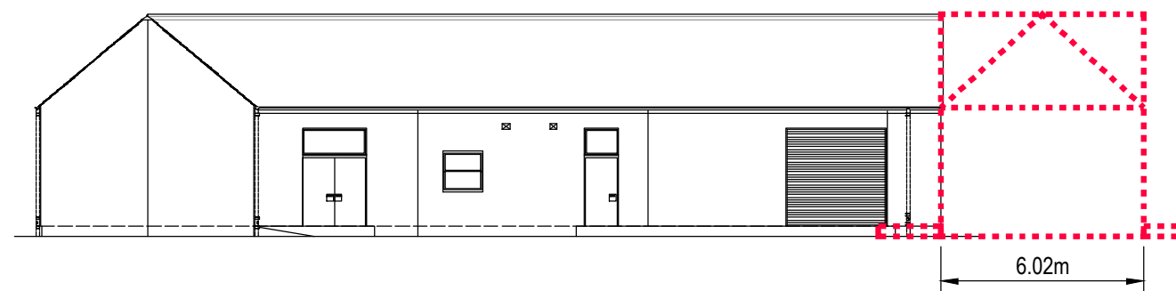
3. REAR ELEVATION
