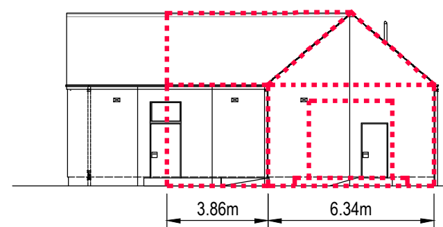
4. SIDE ELEVATION
