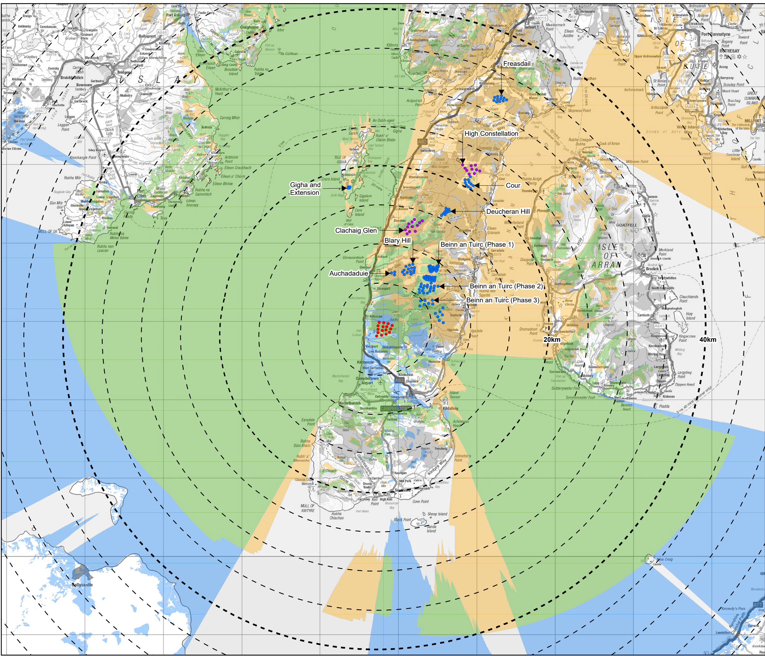
Figure V3a-5.13 Cumulative ZTV - Proposed Varied Development with All Operational and Consented Sites Tangy IV Wind Farm S36C EIA Report 2026 Proposed Varied Development
