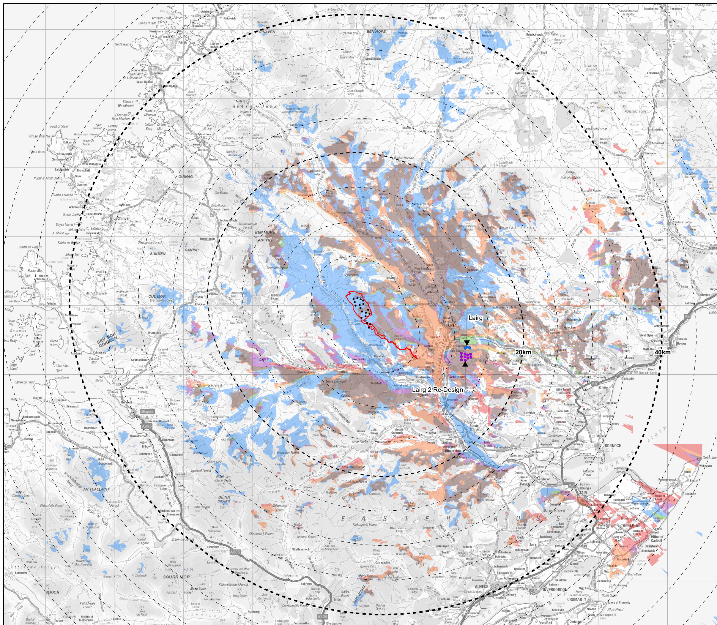
Figure 5.16 Cumulative ZTV - Proposed Varied Development with Lairg and Lairg 2 Re-Design
