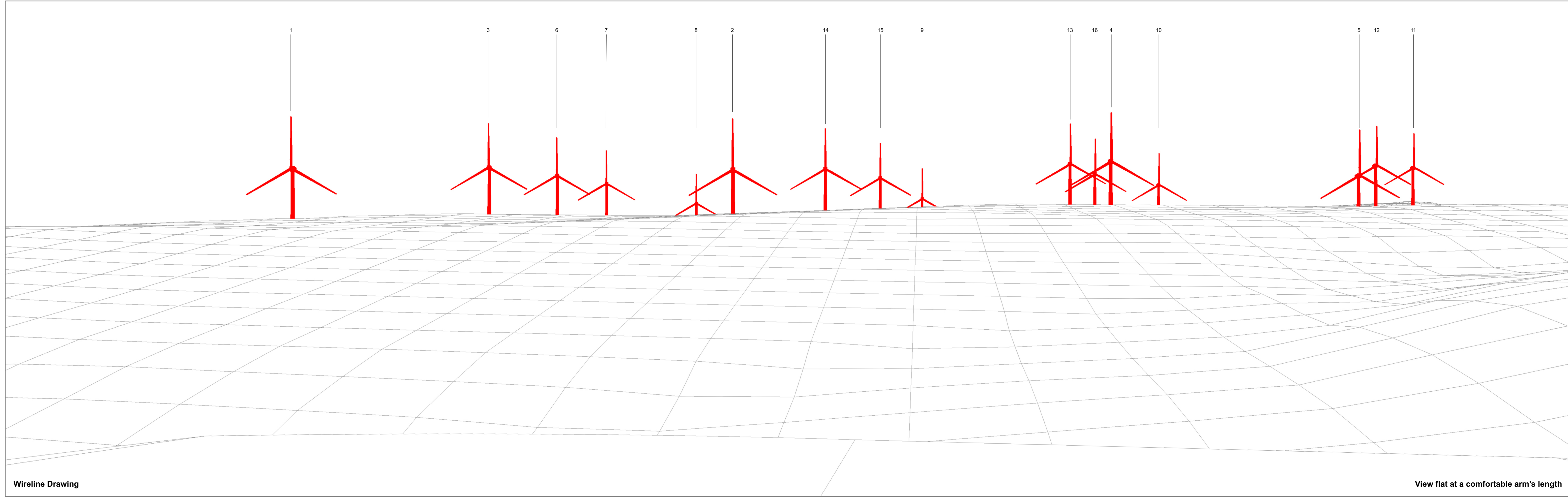
Tangy IV Wind Farm: S36C EIA Report 2026 - Proposed Varied Development Figure V3b 10.17.1 Cultural Heritage Viewpoint 14: Largiemore, fort NE of (SM3063) - Proposed Varied Development Wireline
