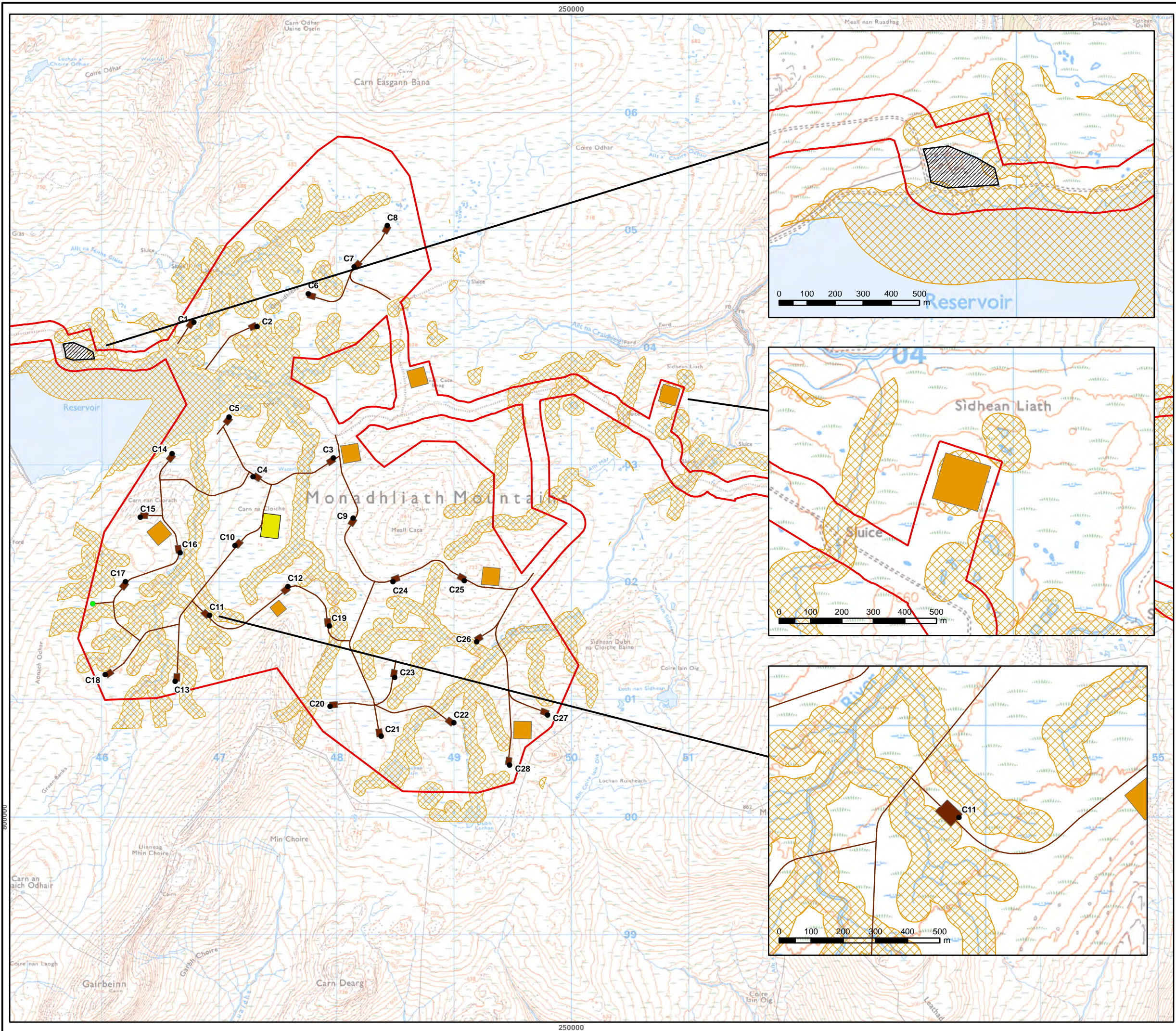
Figure 10.7 Infrastructure within 50m Surface Water Buffer Cloiche Wind Farm EIA Report
