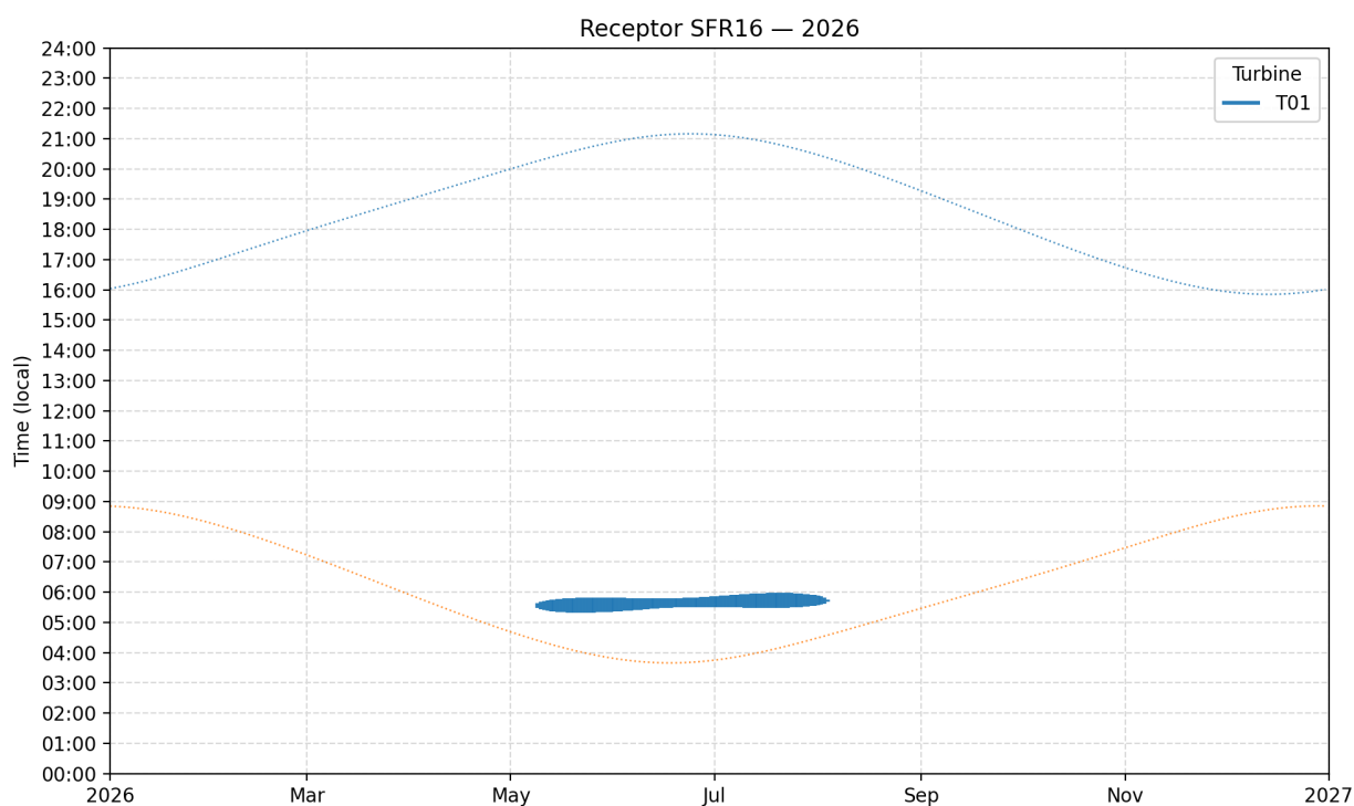
Plate 5: Predicted Shadow Flicker Times at Tangy Glen Cottage - SFR16
