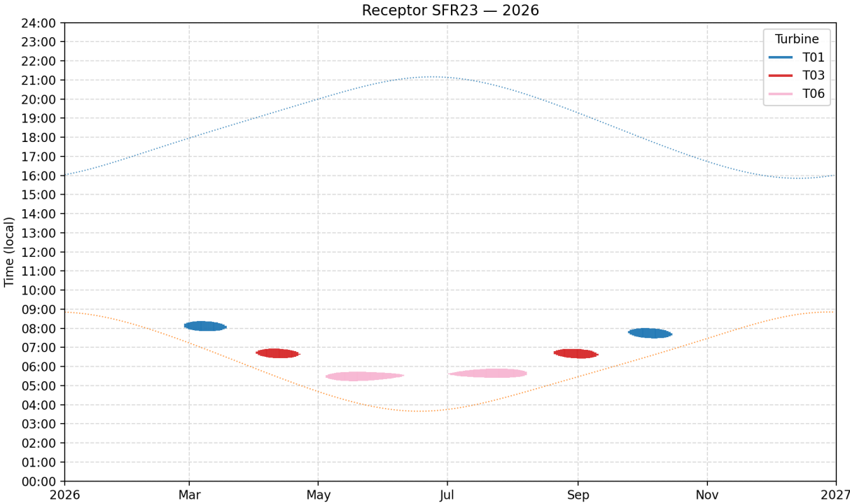
Plate 12: Predicted Shadow Flicker Times at Tighnamoile - SFR23
