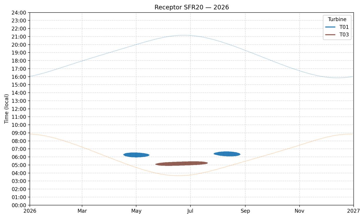
Plate 9: Predicted Shadow Flicker Times at Kilarow Farm - SFR20
