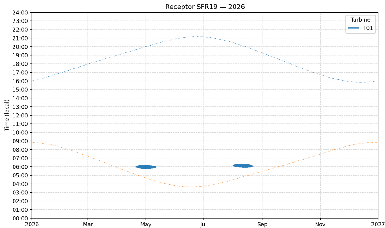
Plate 8: Predicted Shadow Flicker Times at Maleen - SFR19
