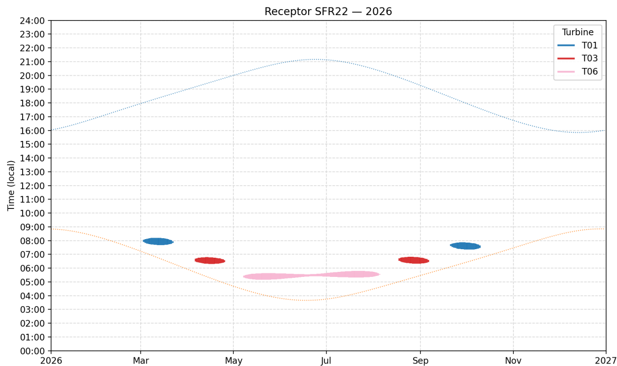
Plate 11: Predicted Shadow Flicker Times at Tangy Moil - SFR22
