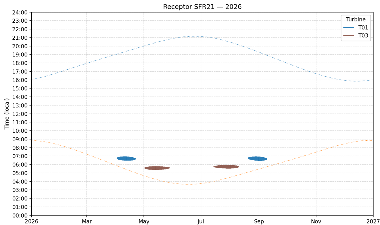
Plate 10: Predicted Shadow Flicker Times at Tigh na Mara - SFR21
