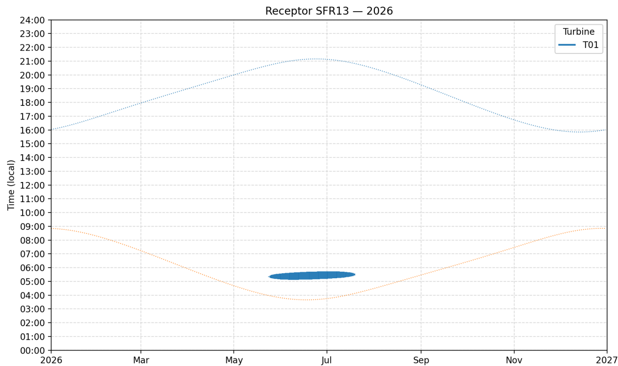
Plate 2: Predicted Shadow Flicker Times at Tangy Mill - SFR13
