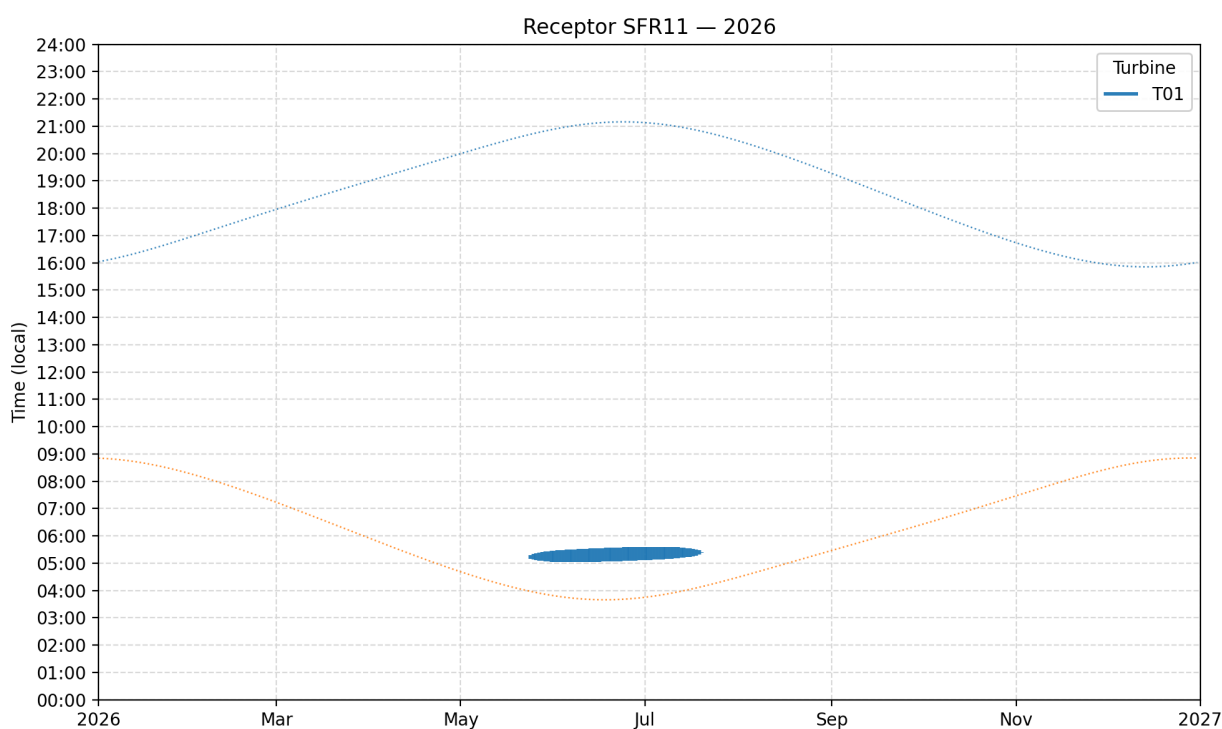
Plate 1: Predicted Shadow Flicker Times at Tangy Mill Croft - SFR11
