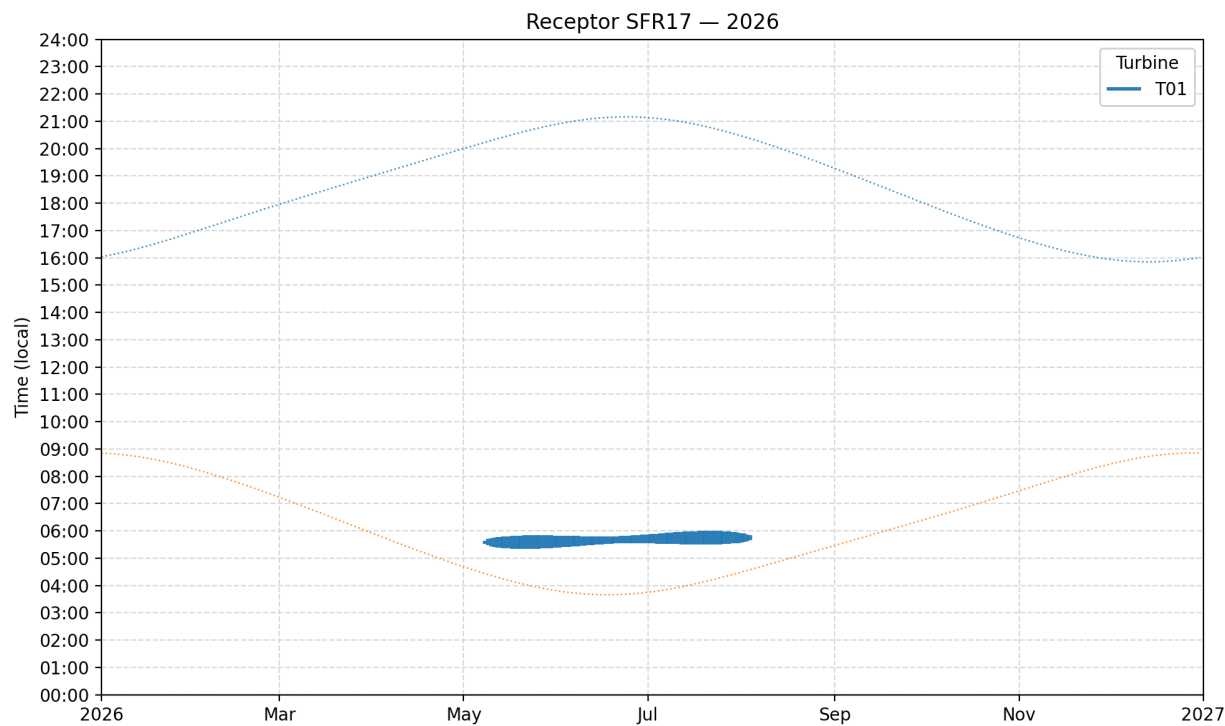
Plate 6: Predicted Shadow Flicker Times at Kilarow Cottage - SFR17
