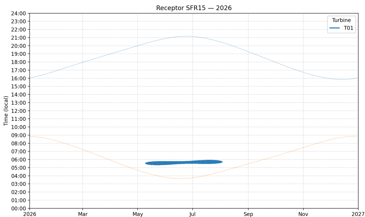
Plate 4: Predicted Shadow Flicker Times at Drumalea Farm Cottage- SFR15
