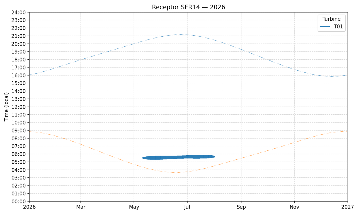
Plate 3: Predicted Shadow Flicker Times at Tangy Smithy - SFR14
