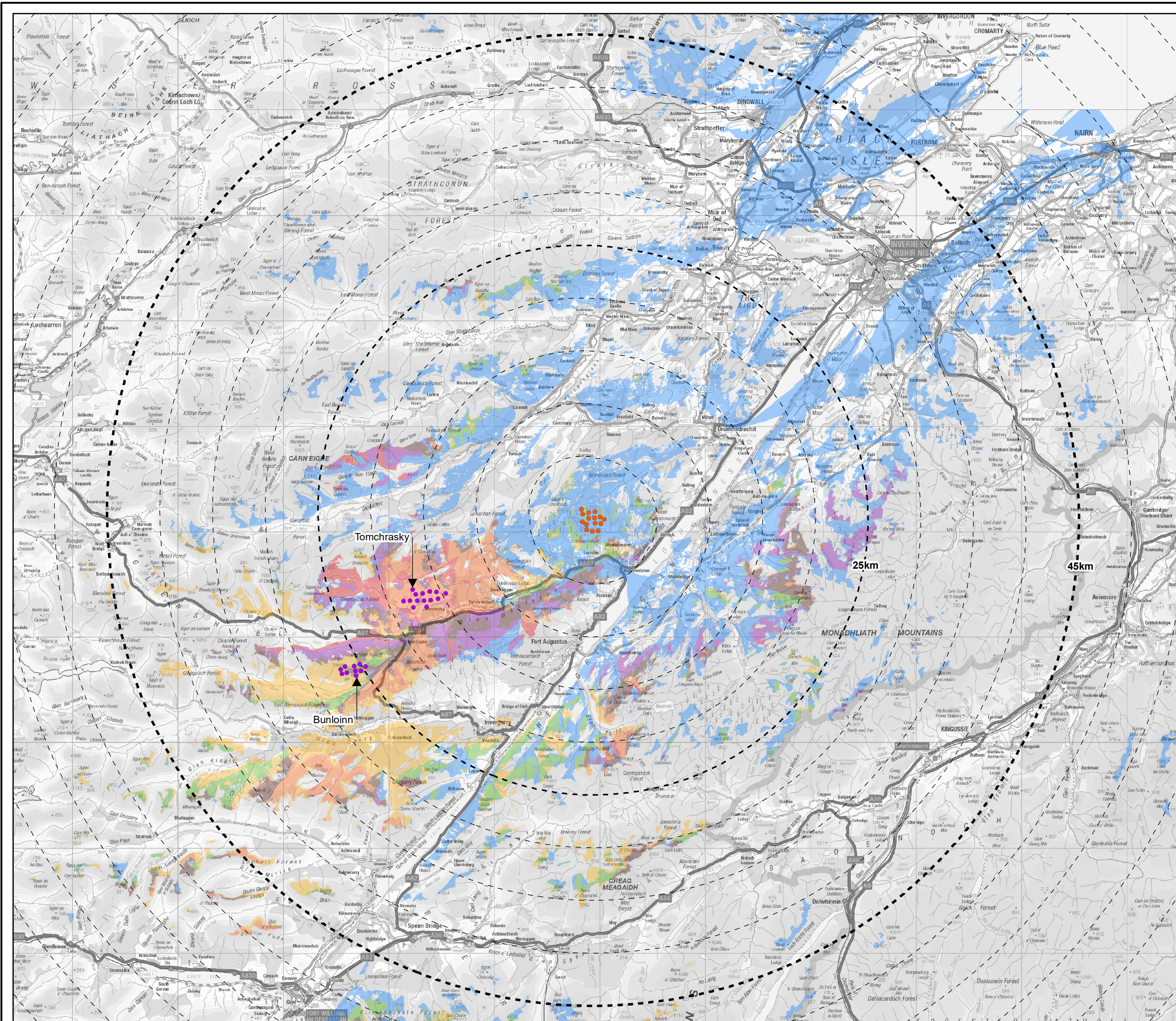
Figure 8.28 Cumulative ZTV - Proposed Varied Development with Bunloinn and Tomchrasky
