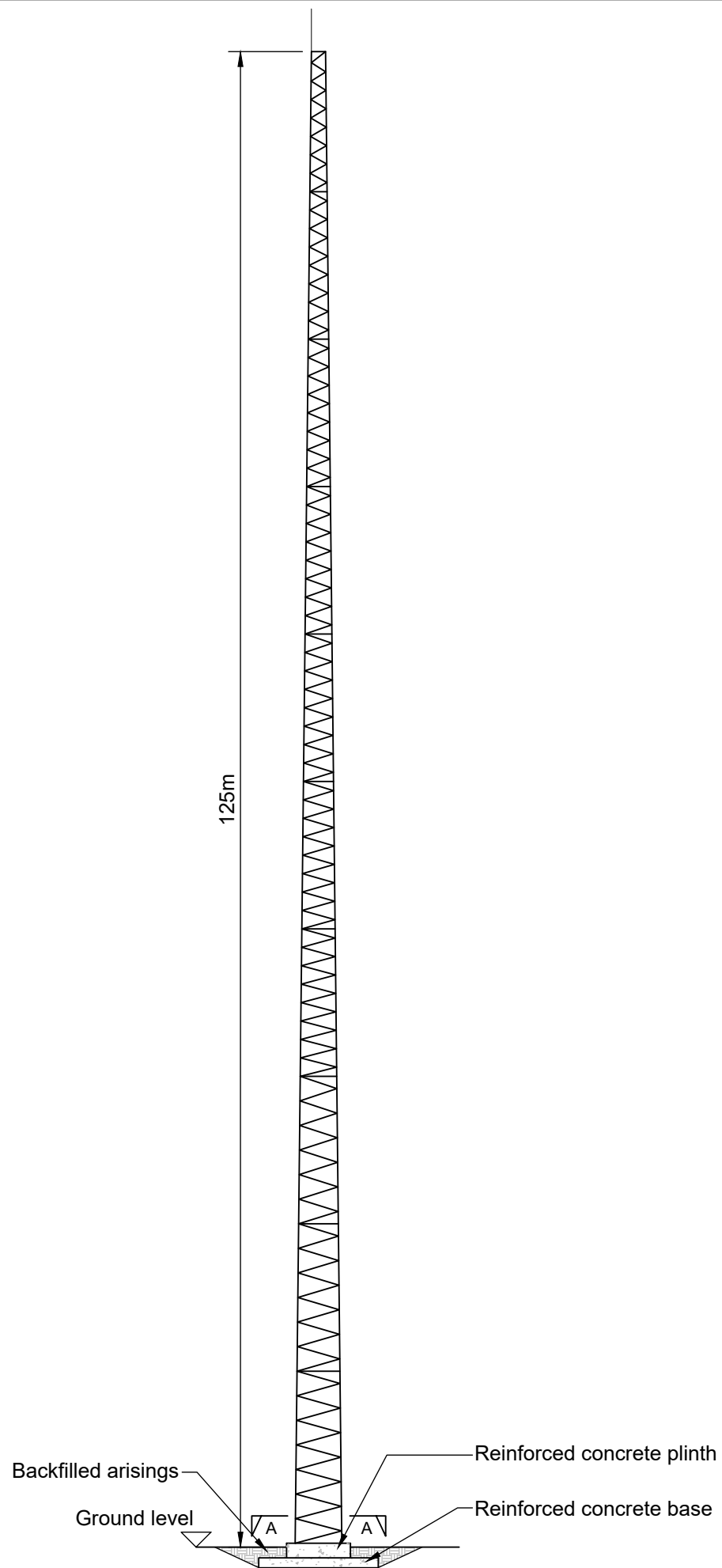
ANEMOMETER MAST ELEVATION Scale 1:500 @ A3
