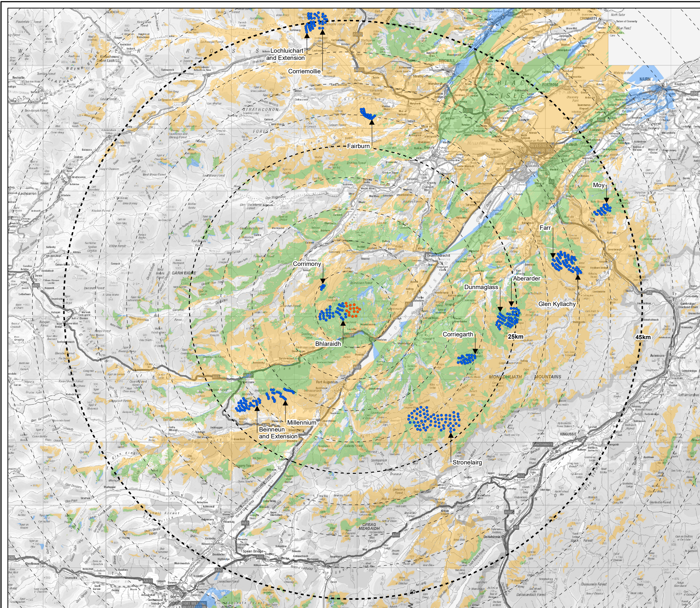
Figure 8.12 Cumulative ZTV - Proposed Varied Development with All Operational Sites
