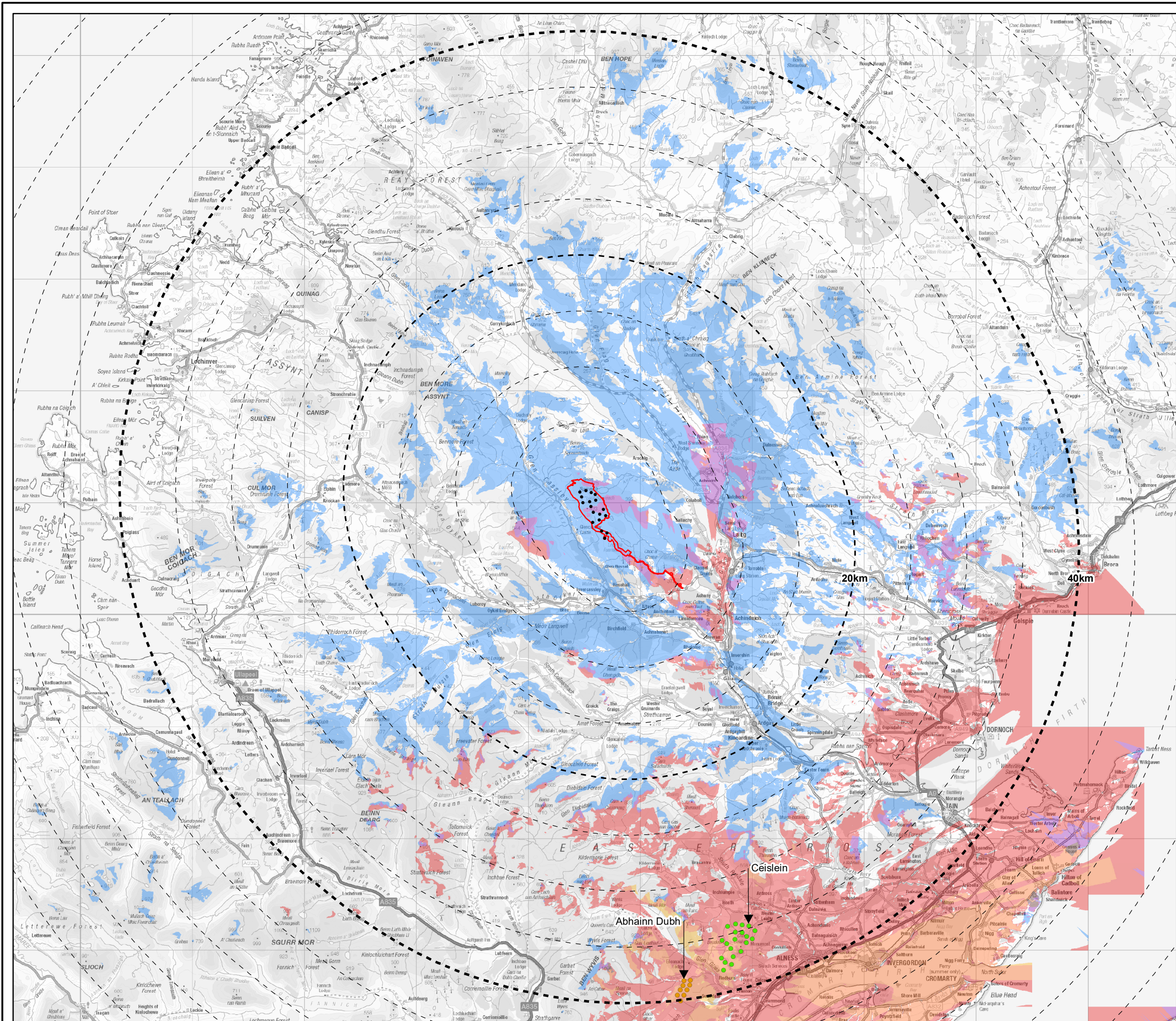
Figure 5.22 Cumulative ZTV - Proposed Varied Development with Abhainn Dubh and Ceislin
