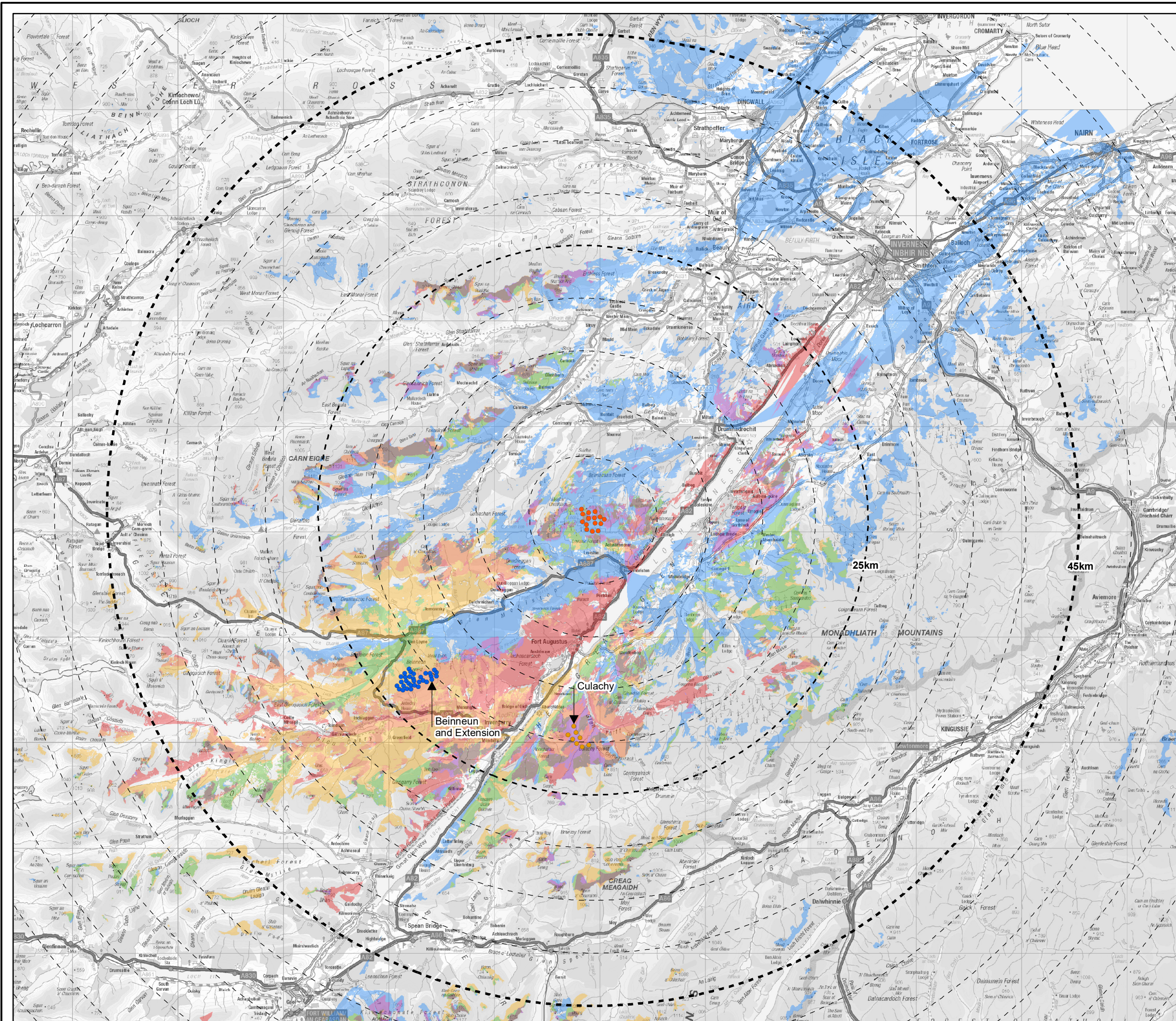
Figure 8.26 Cumulative ZTV - Proposed Varied Development with Beinnneun and Extension and Culachy
