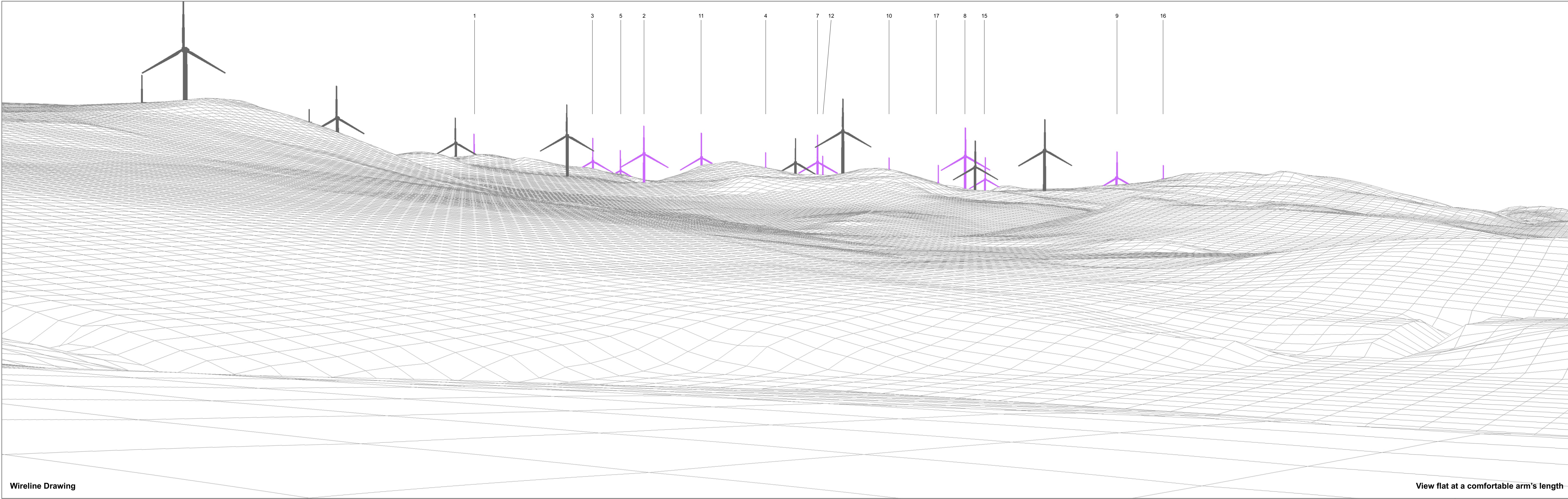
Bhlaraidh Wind Farm Extension Section 36C: EIA Report Figure V3a 1.3b - Viewpoint 1: Track to Loch Liath - Consented Development Wireline
