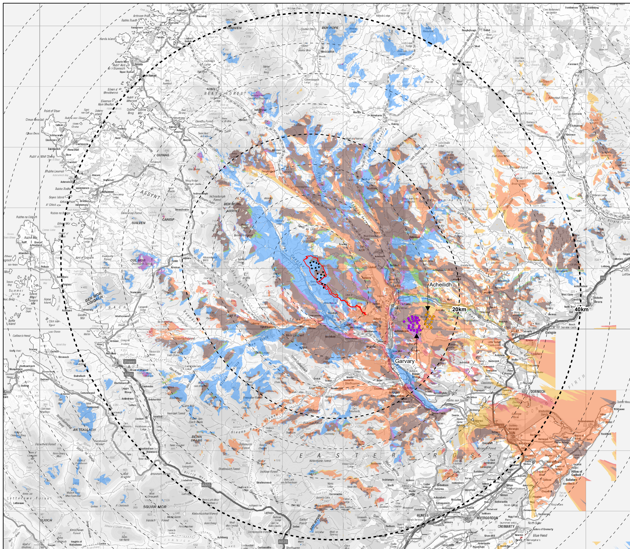
Figure 5.16 Cumulative ZTV - Proposed Varied Development with Acheilidh and Garvary
