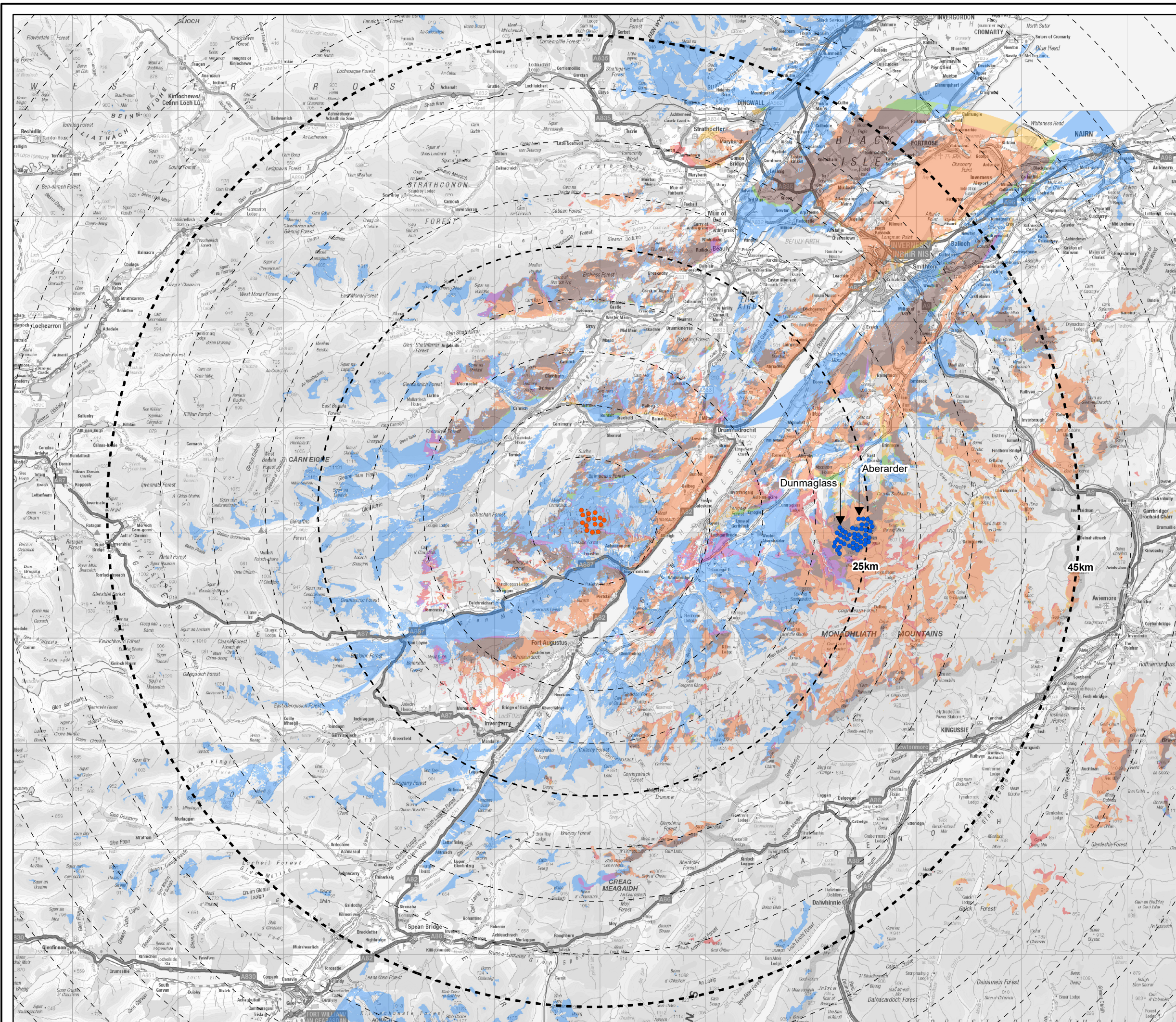
Figure 8.22 Cumulative ZTV - Proposed Varied Development with Aberarder and Dunmaglass Bhlaraiddh Wind Farm Extension Section 36C: EIA Report
